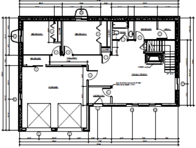
BASMENT FLOOR PLAN SCALE 1/4" = 1'-0"
