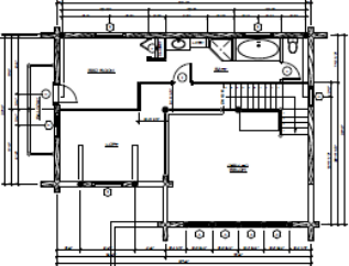
SECOND FLOOR PLAN SCALE 1/4" = 1'-0"
